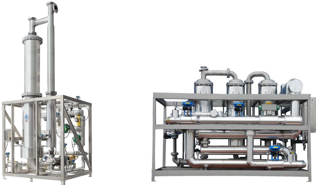
Illustration 4: Vertical configuration (left) and horizontal configuration (right) of the ProFlow continuous enzymatic conversion system.
