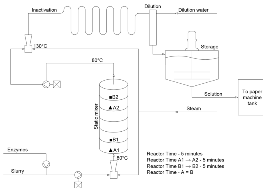
Illustration 1: The plug flow principle minimizes viscosity fluctuations.
